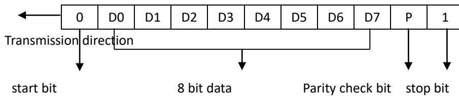
Figure 1 byte transmission sequence
